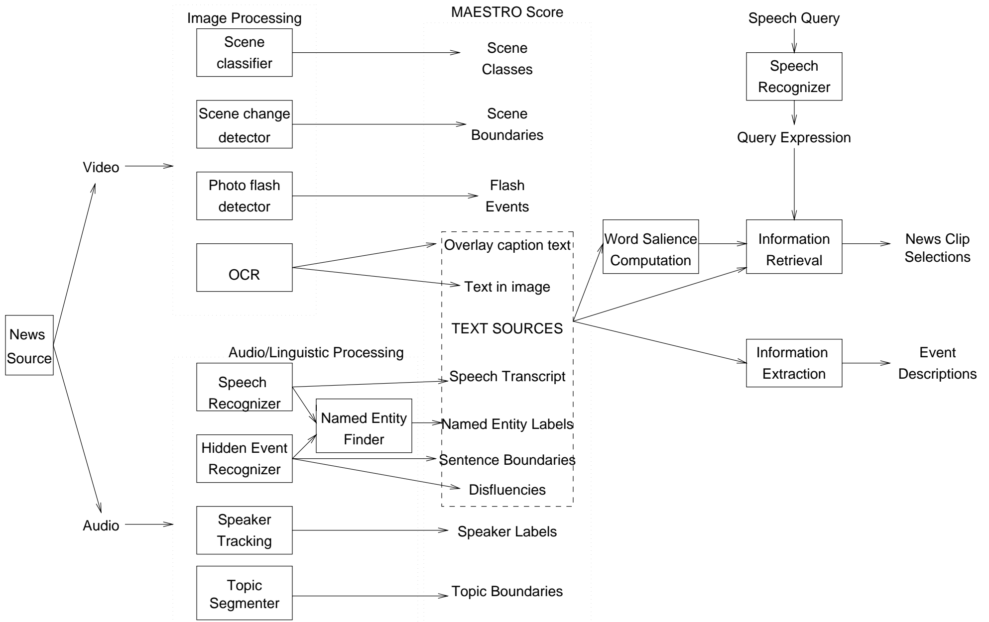
SRI News-On-Demand System (MAESTRO)
